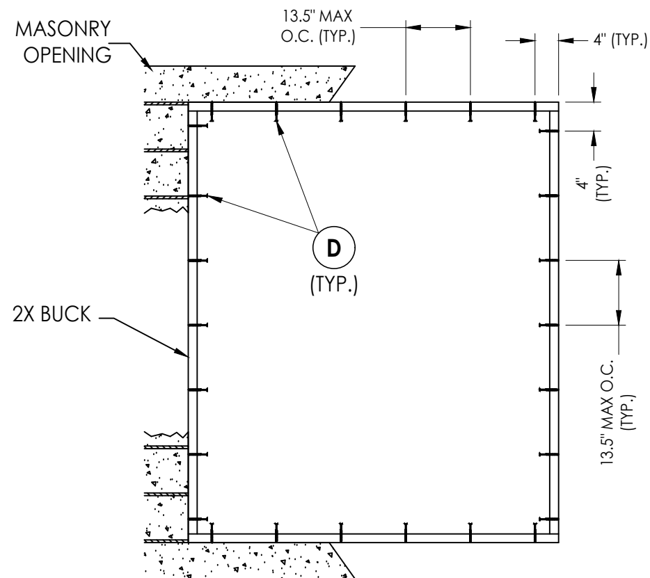
BUCK ANCHORING MASONRY
