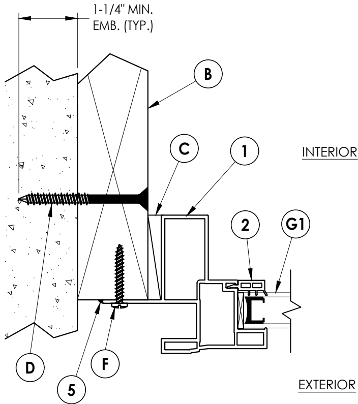
1 2 HORIZONTAL CROSS SECTION
